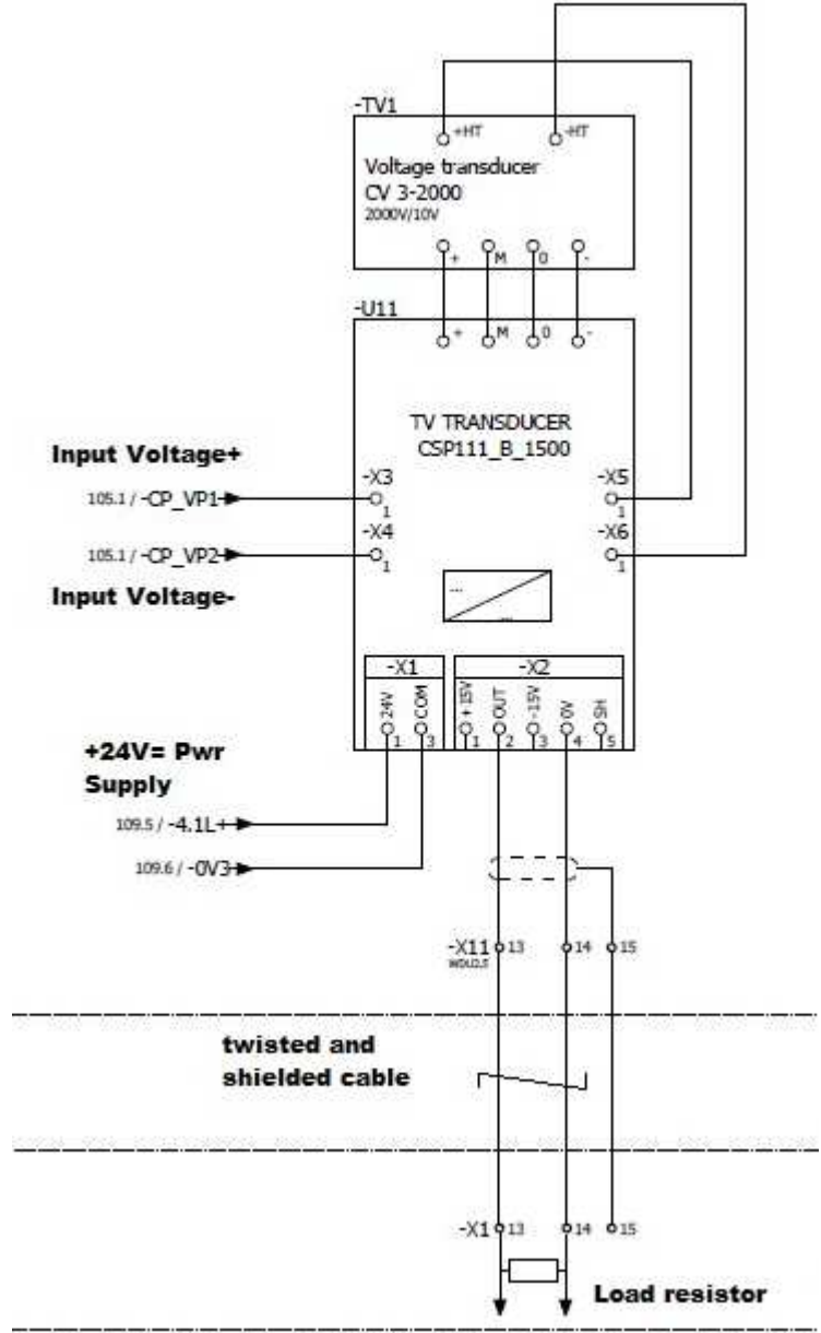
Fig. 2 - CSP111B example of connection
